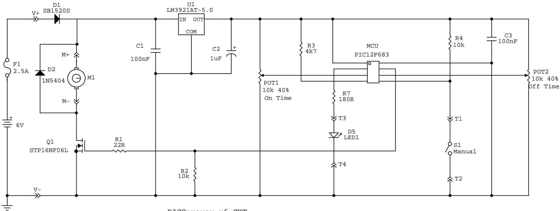
PICSprayer_r6.CKT July 2011
