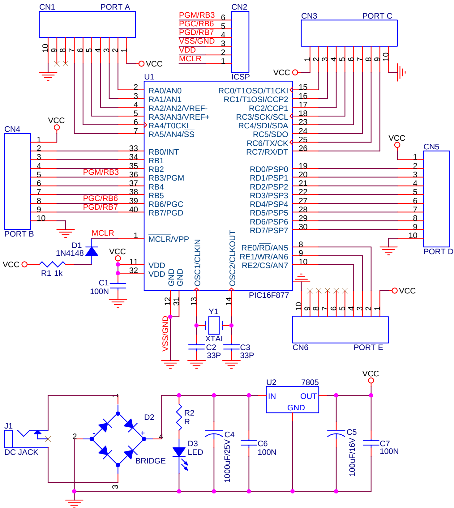
PIC DEVELOPMENT BOARD - 16F877
